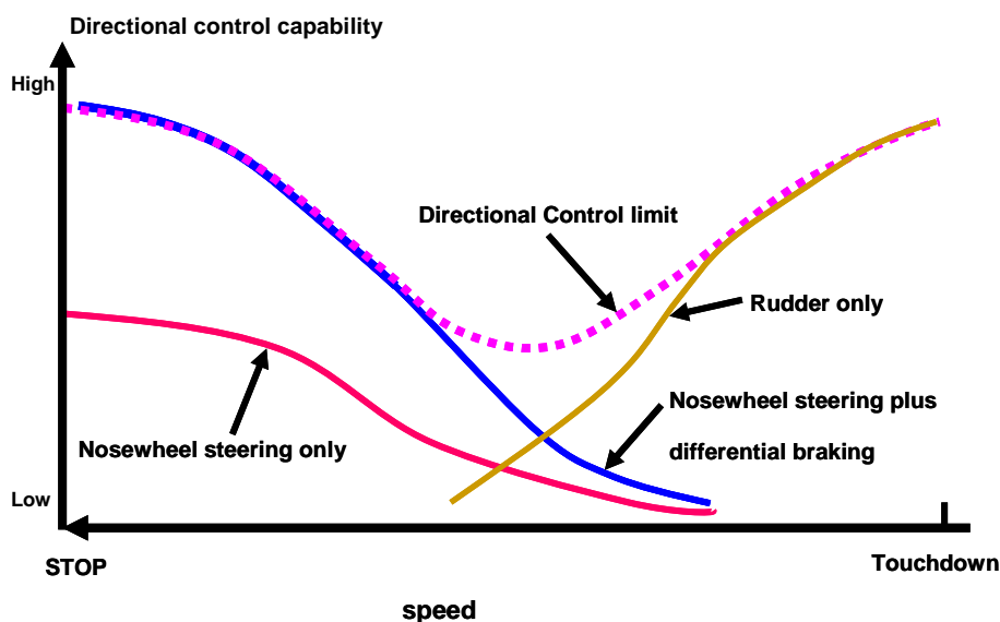
Figure 6: Influence of nose wheel steering, differential braking, and rudder on ground directional control
